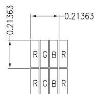
PIXEL DETAIL (SCALE 40:1)
