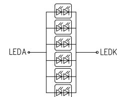
BACKLIGHT CIRCUIT DIAGRAM
